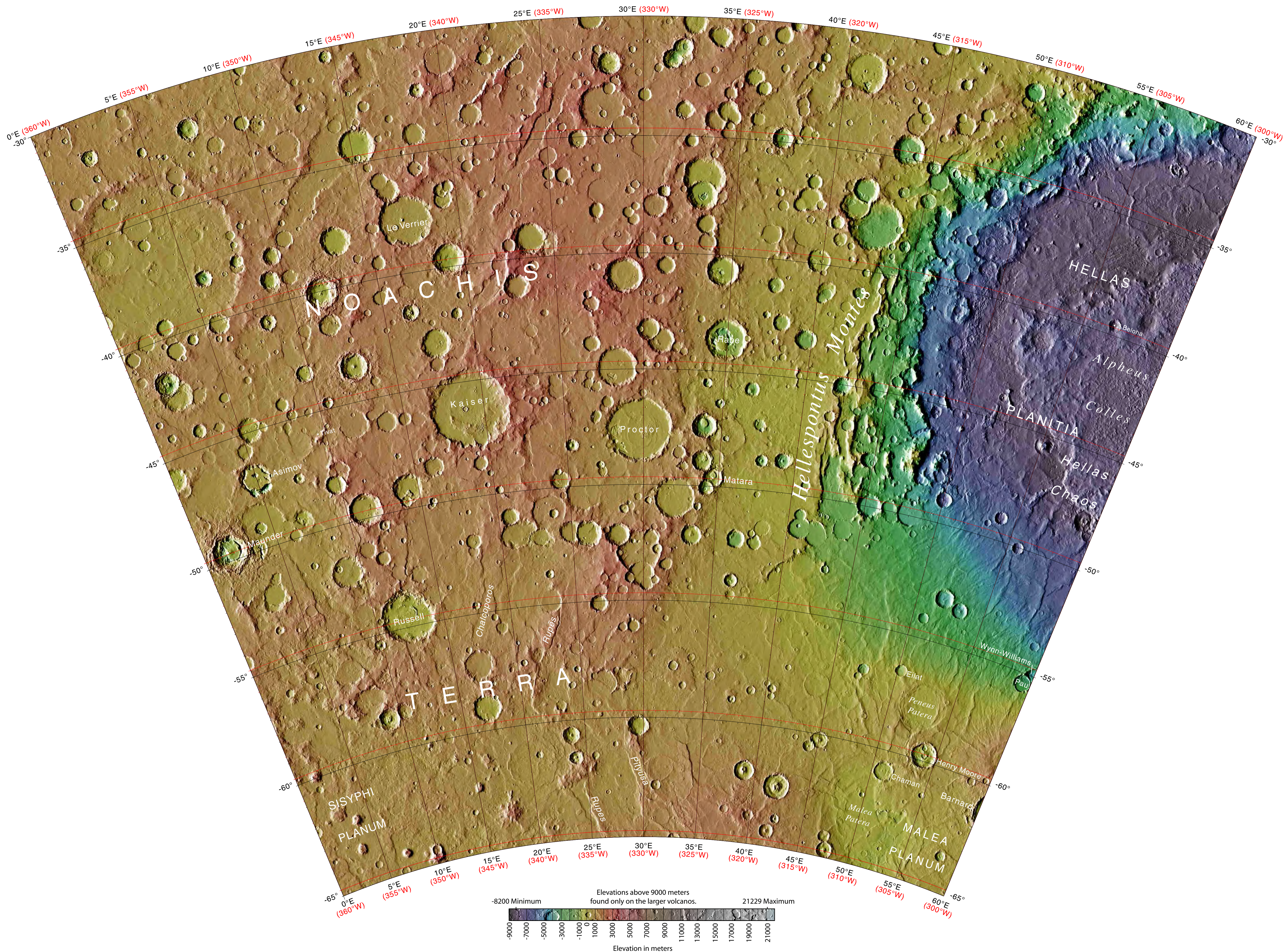
Noachis, MC-27 Lambert Conformal Conic Projection
