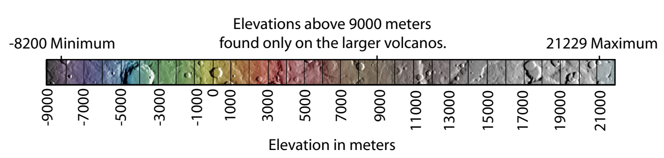
Argyre, MC-26 Lambert Conformal Conic Projection
