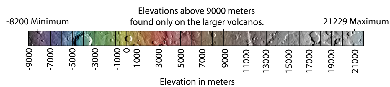
Memnonia, MC-16 Mercator Projection
