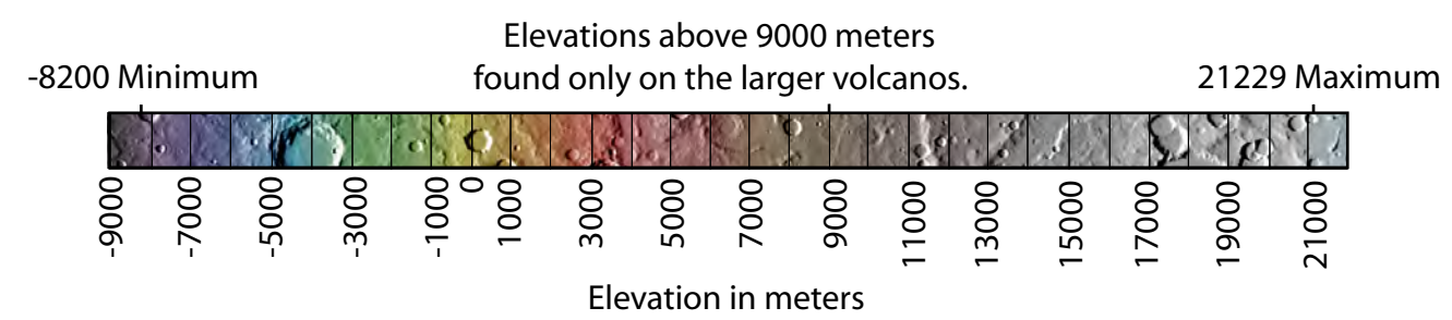
Amenthes, MC-14 Mercator Projection
