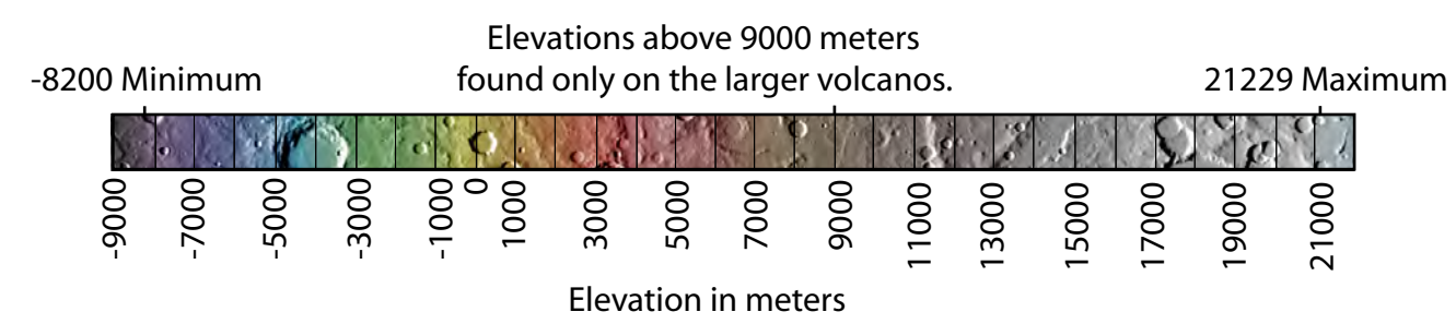
Amazonis, MC-8 Mercator Projection
