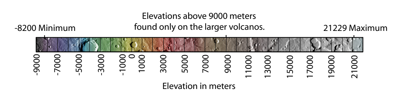
Mare Acidalium, MC-4 Lambert Conformal Conic Projection
