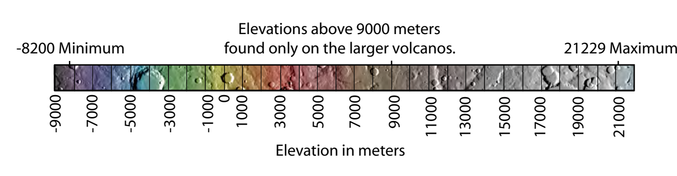
Arcadia, MC-3 Lambert Conformal Conic Projection
